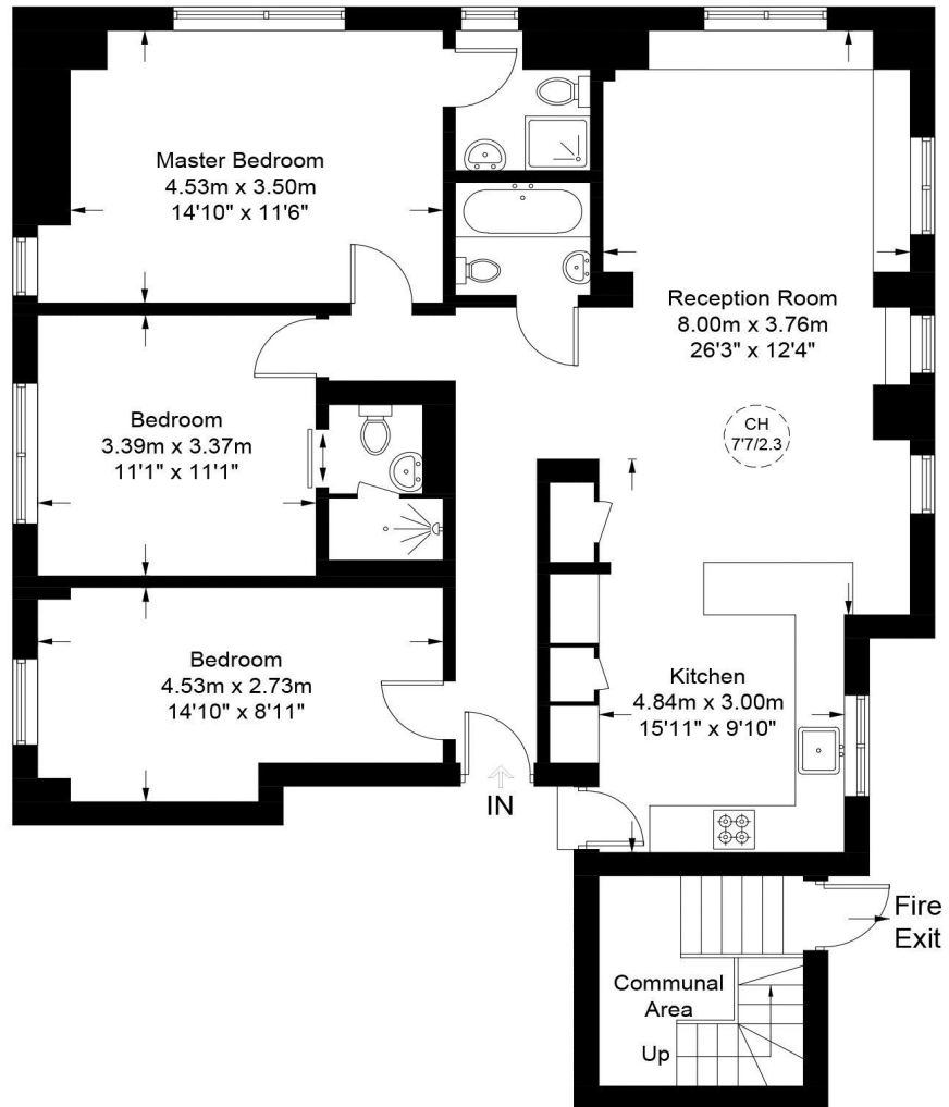
Fifth Floor
