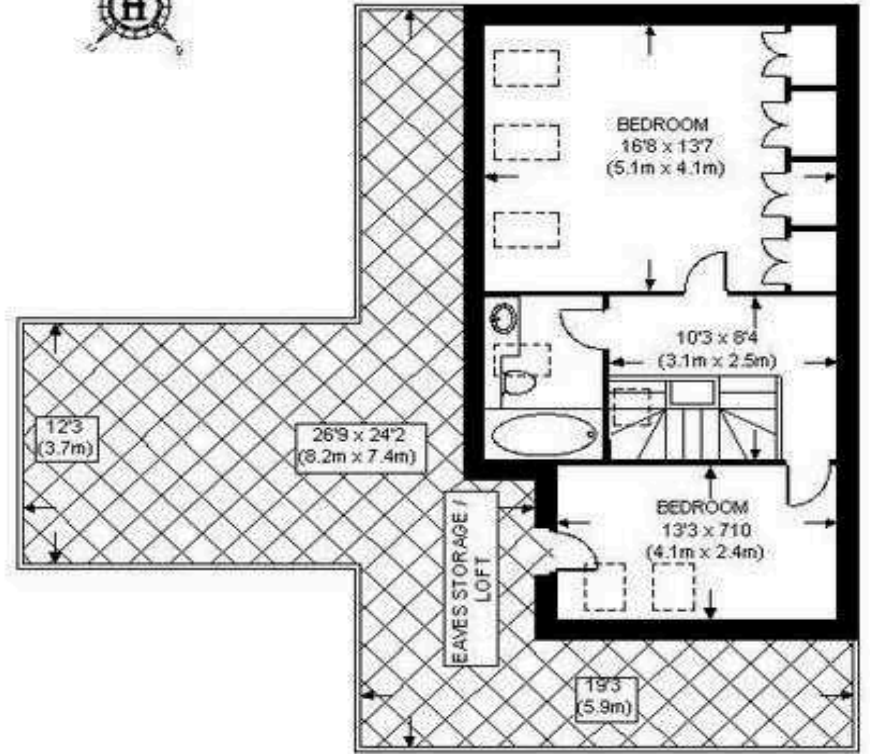
THIRD FLOOR
