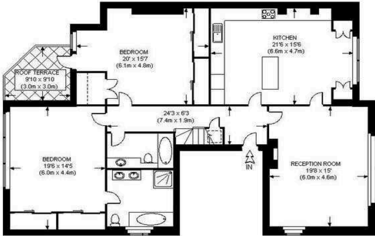
SECOND FLOOR
